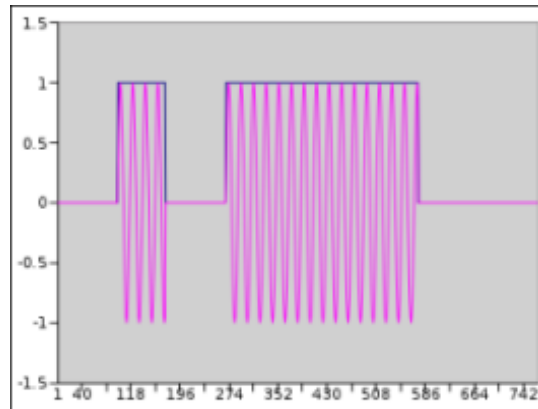
Figure 2.114 Dash/Dot = 4.0, Edge = 0.0
