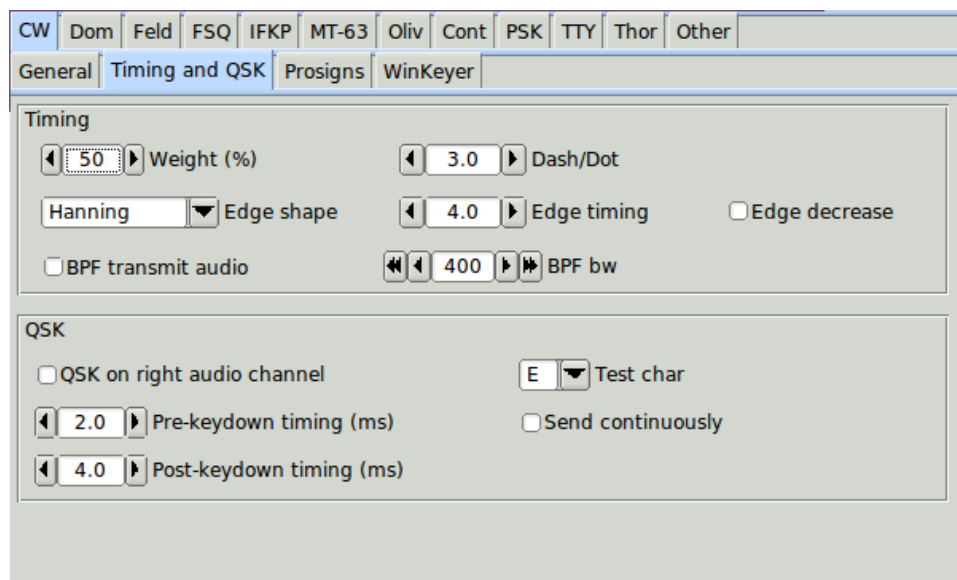
Figure 2.112 Timing
