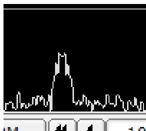
Figure 2.17 FFT
