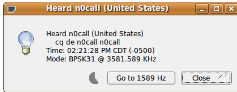
Figure 6.72 Notifier Popup
