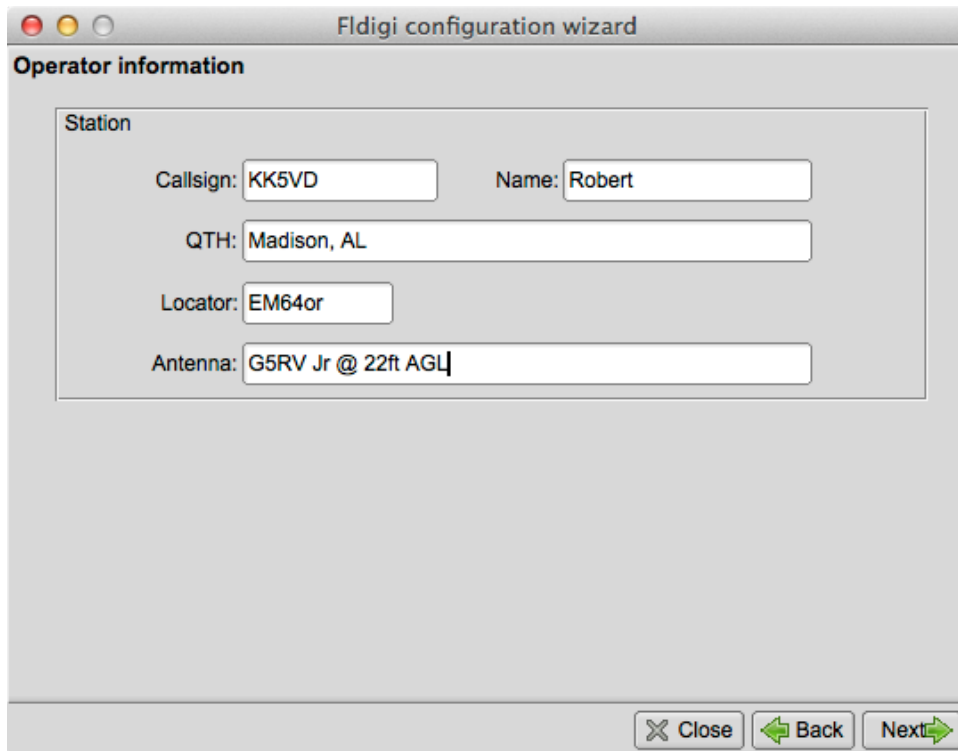
Figure 2.38 Operator Configuration
