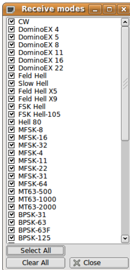
Figure 2.123 Receive Modes
