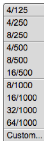
Figure 6.46 Contestia
