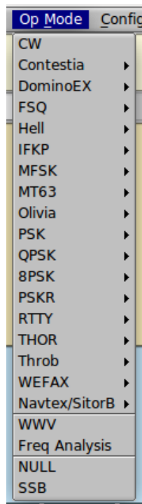
Figure 6.45 Op Mode
