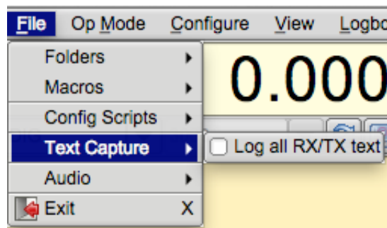
Figure 6.41 Text Capture
