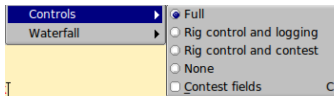
Figure 6.64 View Controls
