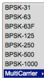
Figure 6.51 PSK
