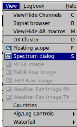
Figure 6.63 View
