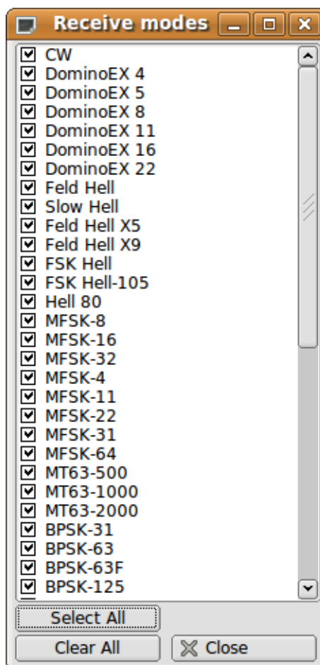
Figure 2.59 Receive Modes
