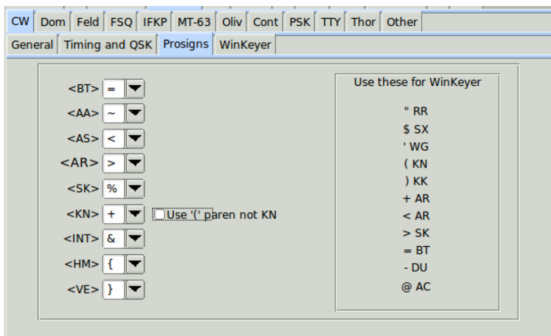
Figure 2.118 CW Prosigns
