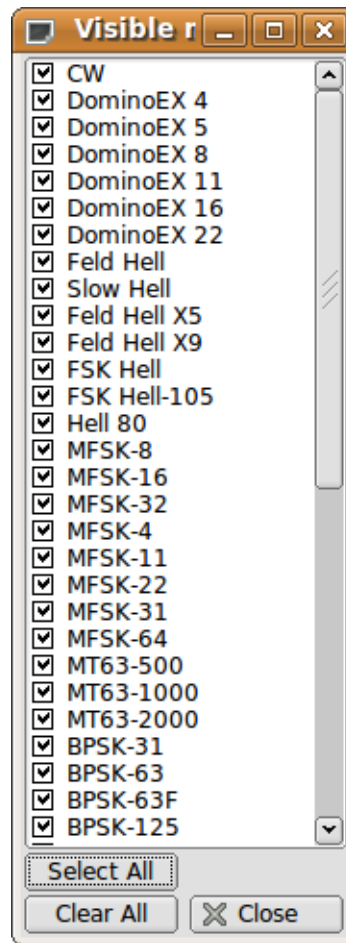
Figure 2.76 Visible Modes
