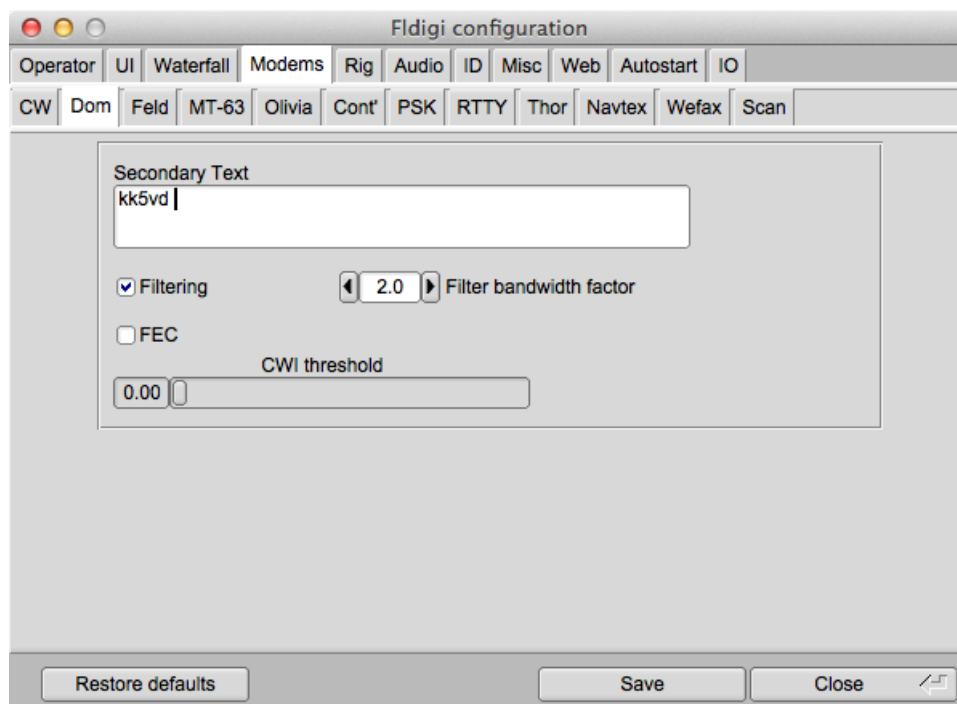
Figure 2.120 DominoEX Configuration
