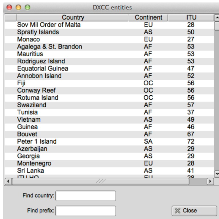
Figure 6.14 DXCC List
