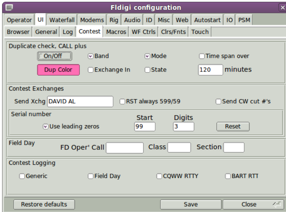
Figure 2.73 UI Contest
