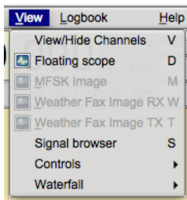
Figure 6.88 View Menu
