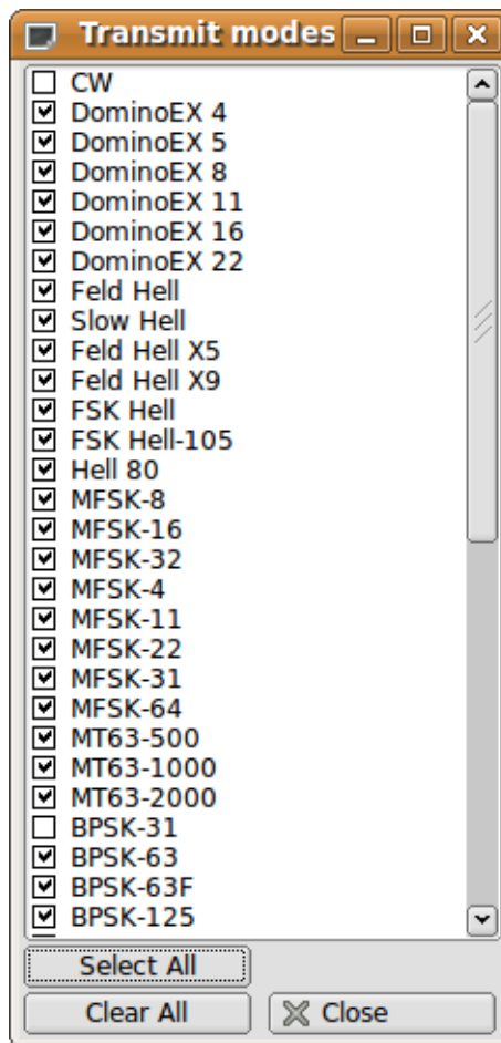
Figure 2.124 Transmit Modes
