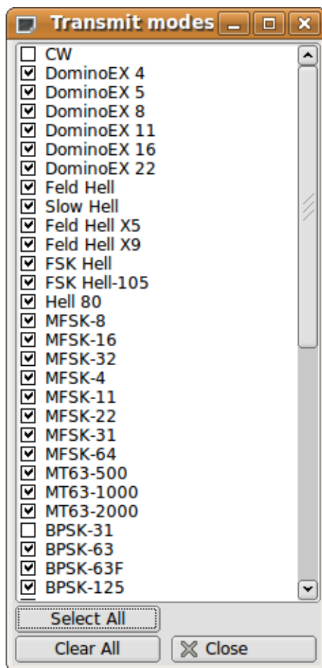
Figure 2.60 Transmit Modes
