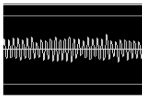
Figure 2.18 Scope
