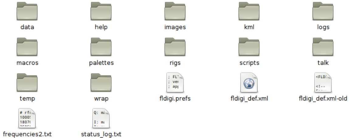
Figure 2.24 Working Folder
