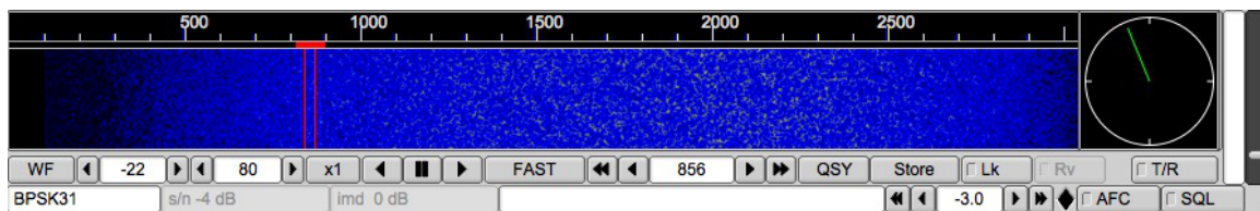
Figure 6.74 FLDIGI Controls
