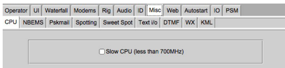
Figure 2.133 Misc CPU
