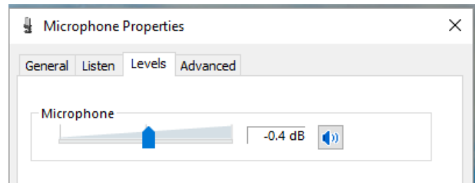
Figure 2.21 Microphone Level
