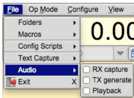
Figure 6.43 Exit
