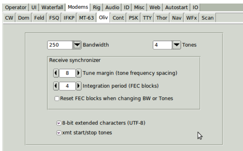
Figure 2.139 Description
