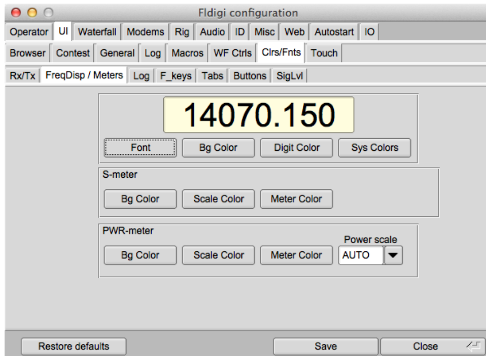
Figure 2.47 Frequency Display
