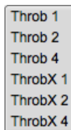
Figure 6.59 throb
