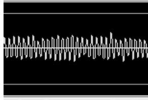
Figure 2.15 Scope view
