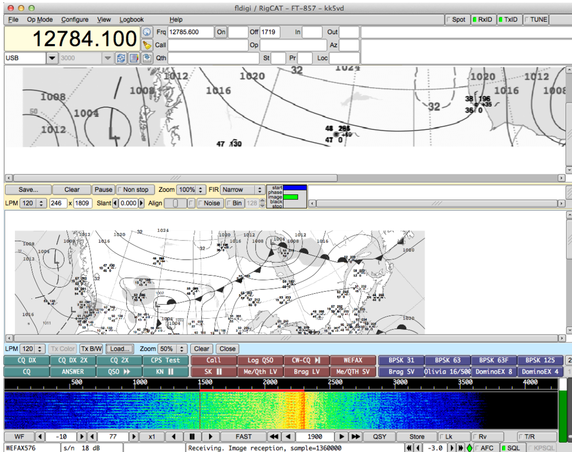
Figure 2.106 Received Image
