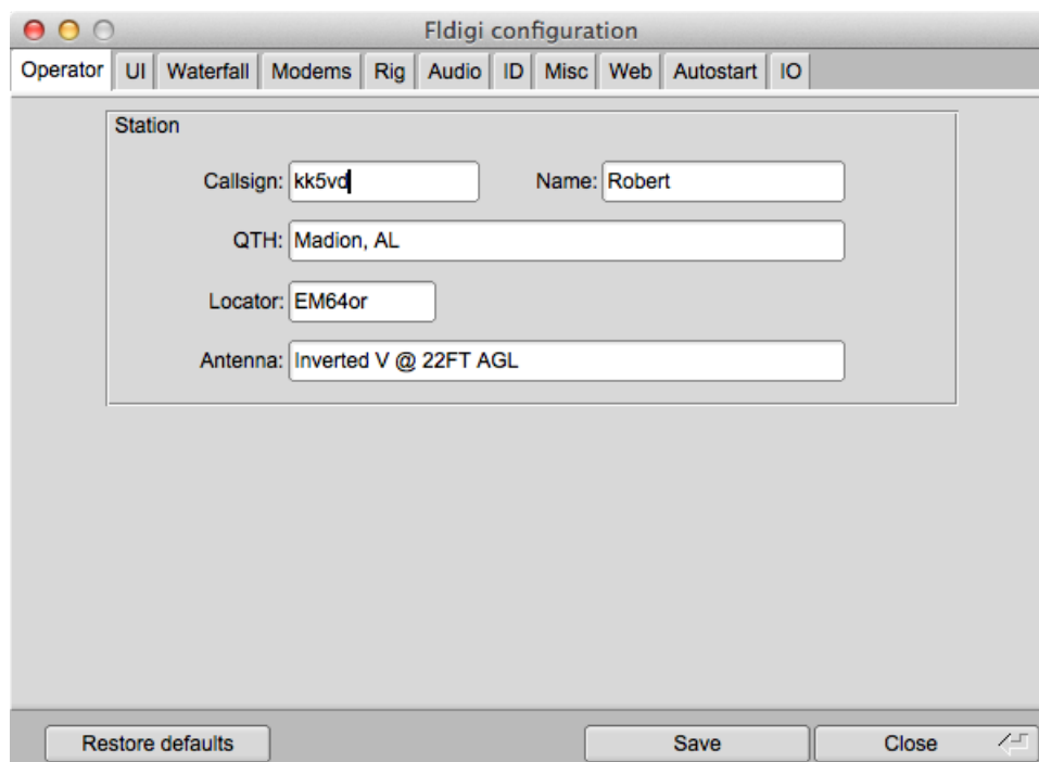
Figure 2.1 Operator
