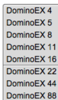
Figure 6.47 DominoEX
