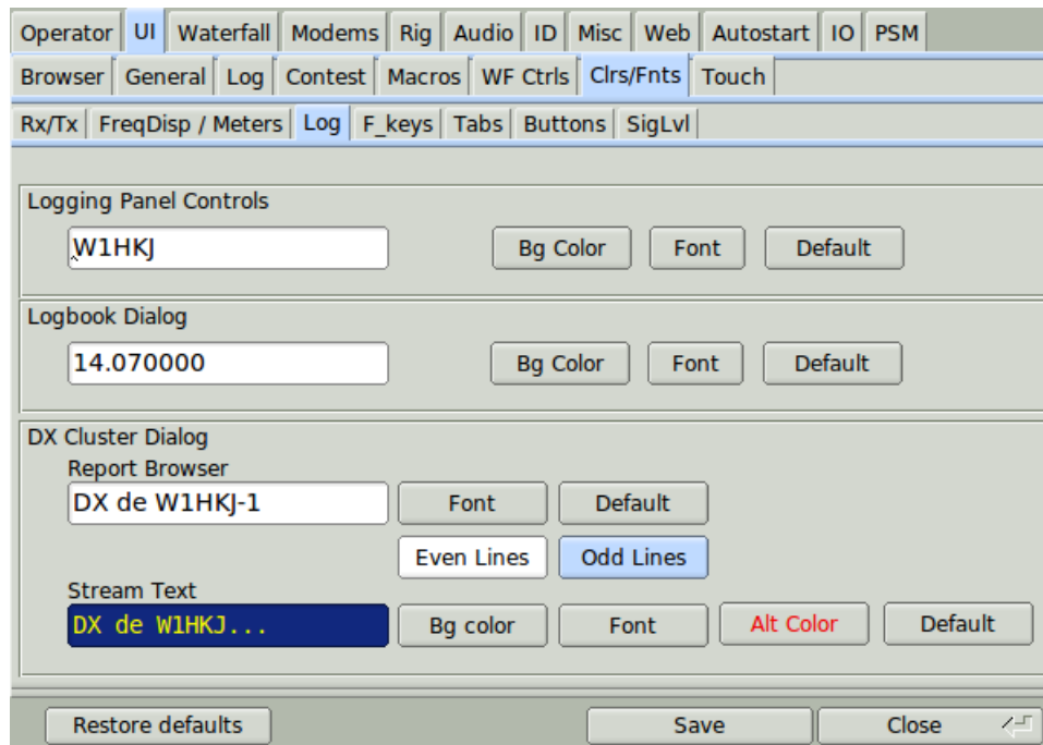
Figure 2.48 Logging controls
