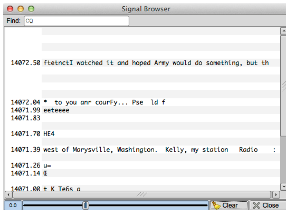
Figure 2.71 Browser Panel
