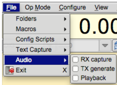
Figure 6.42 Audio
