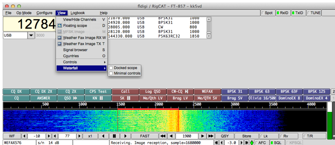
Figure 2.96 WEFAX
