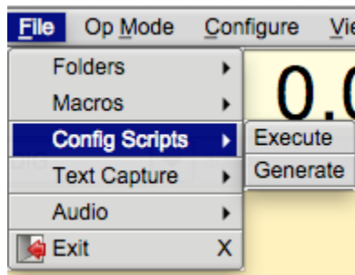
Figure 6.44 Config Scripts
