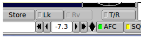
Figure 6.81 TX level
