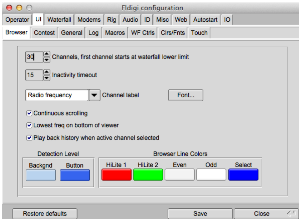
Figure 6.91 Browser Configure
