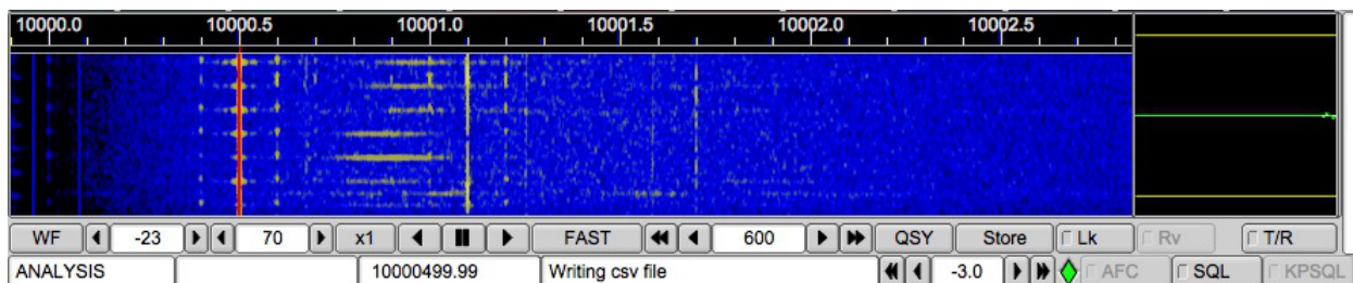
Figure 6.15 Frequency Analyzer
