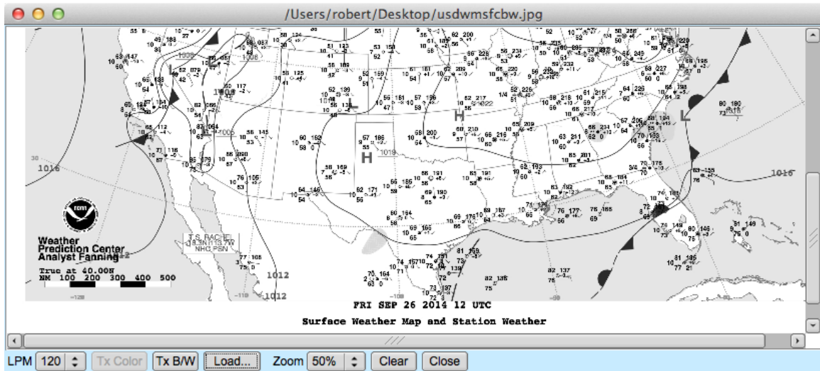
Figure 2.100 Sending
